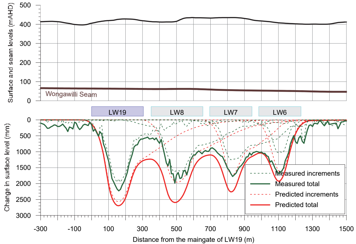
Fig. 2.11 Measured changes in surface level and predicted vertical subsidence along Cross-section 2
