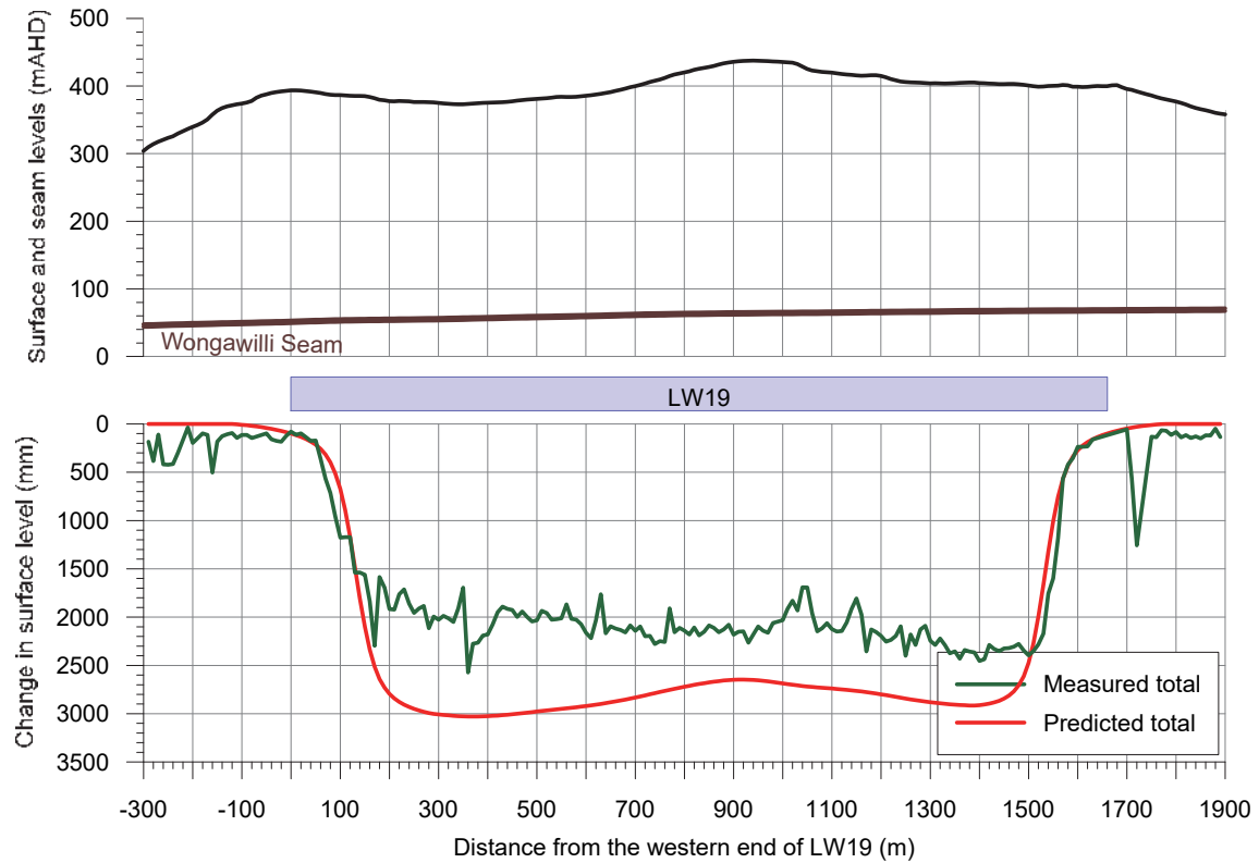
Fig. 2.13 Measured changes in surface level and predicted vertical subsidence along Long-section 1
