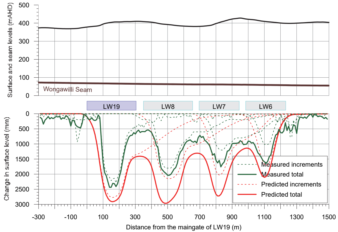
Fig. 2.12 Measured changes in surface level and predicted vertical subsidence along Cross-section 3
