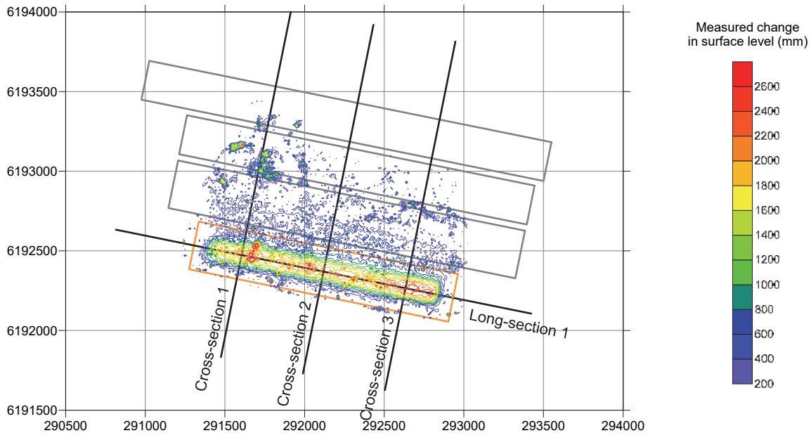
Fig. 2.8 Measured incremental changes in surface level due to the mining LW19
