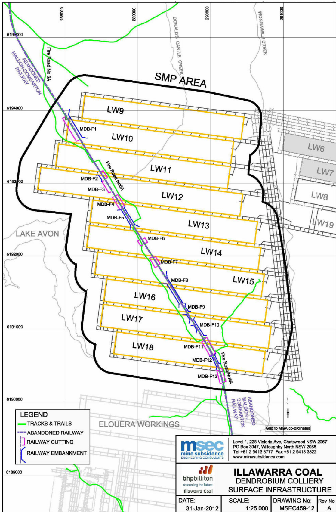
Drawing MSEC459-12
